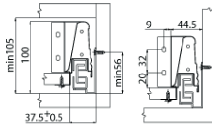
Assembling dimensions of cabinet // Drawer back
