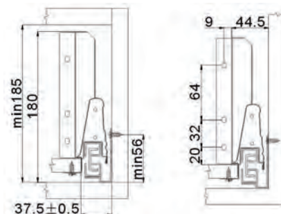
Assembling dimensions of cabinet//Drawer back
