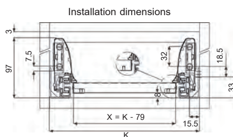
Installation dimensions
